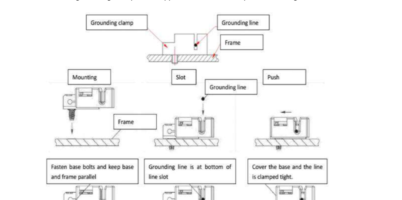
Figure 6 Grounding Clamp Installation
